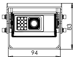
FRAME DRAWING
