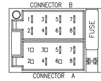
ISO CONNECTOR 4PIN+8PIN FEMALE WITH MALE TERMINAL
